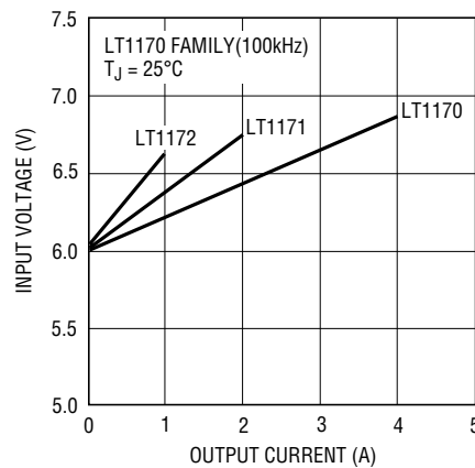
Minimum Input Voltage – Normal Mode (1170 Family)
