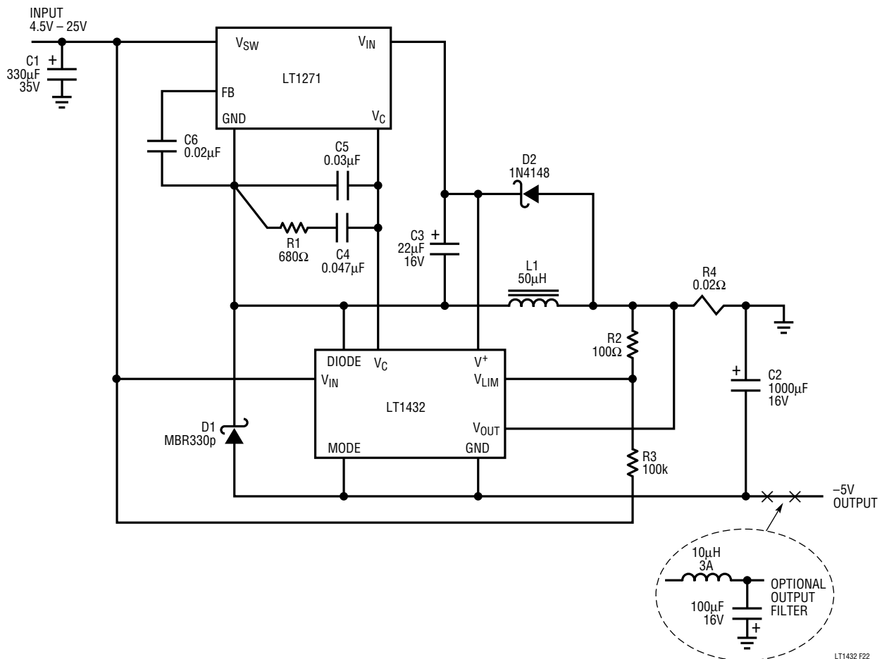
Figure 22. Positive-to-Negative Converter
